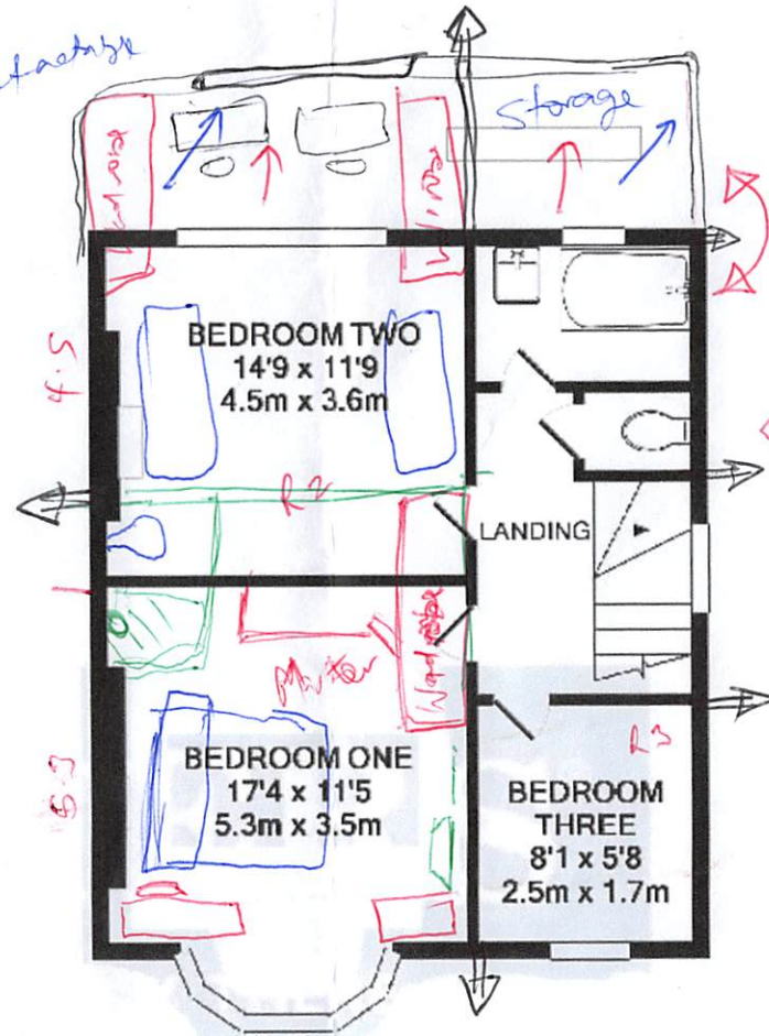
5.2 1ST FLOOR
